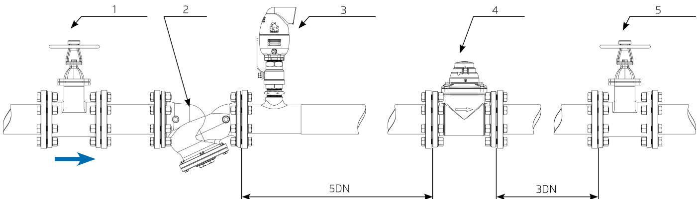
[1] Isolation Valve
