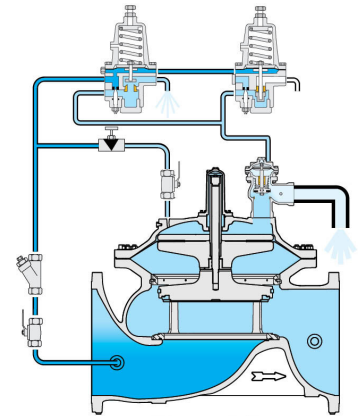
H.P. regeling
