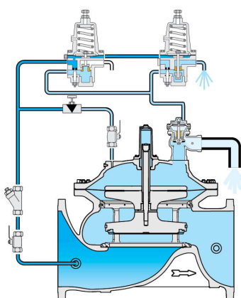
L.P. Regulating
