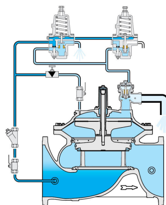
H.P. Regulating
