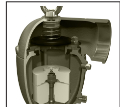
With Inflow Prevention (C75-IP)
