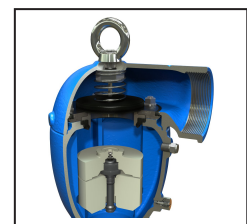
With Inflow Prevention (C75-IP)
