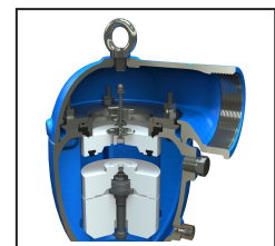
With Assisted Closing (C75-AC)
