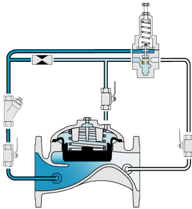
Pressure Relief
