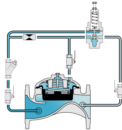
Pressure Sustaining
