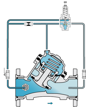
Pressure Sustaining
