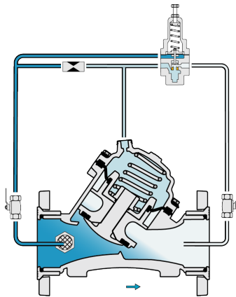
Pressure Relief
