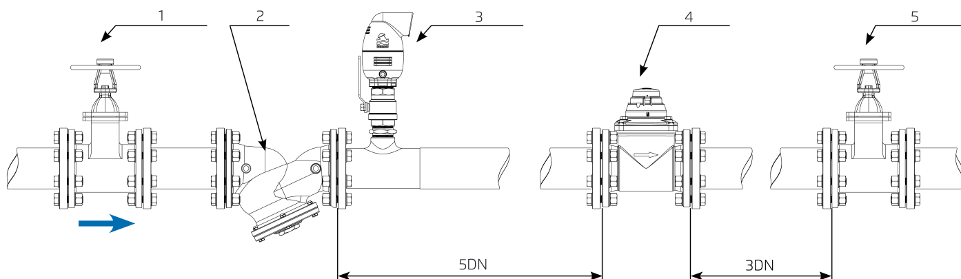
[1] Isolation Valve
