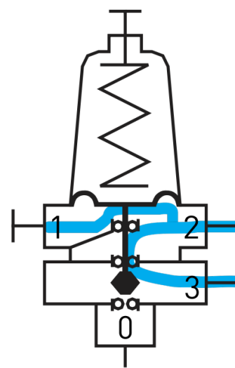
Modulating Open Regulated pressure lower than setting: 3 <--> 1, 2
