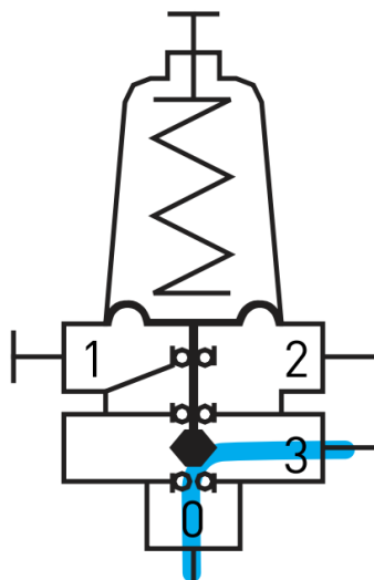
Modulating close Regulated pressure higher than setting: 0 <--> 3
