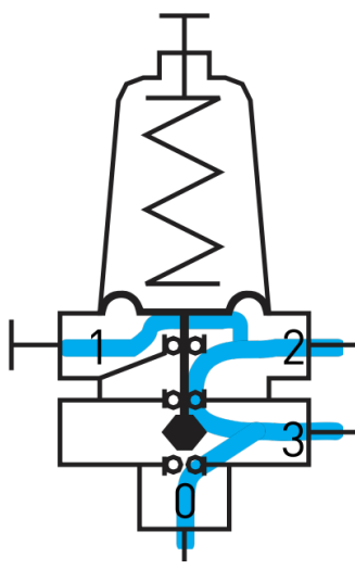
Stable Position Regulated pressure equal to setting: 0 <--> 3 <--> 1, 2 controlled passage
