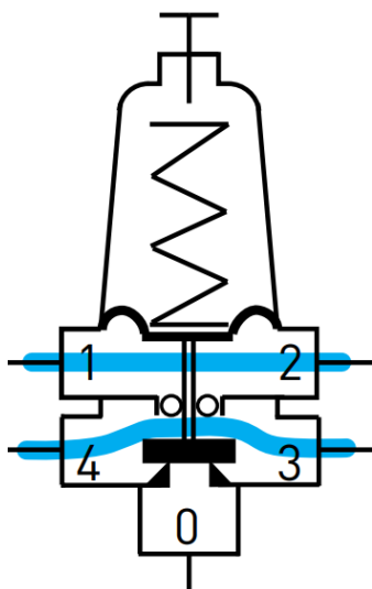
Modulating close Regulated pressure Lower than setting: 4 \leftrightarrow 3 \mid \leftrightarrow 0
