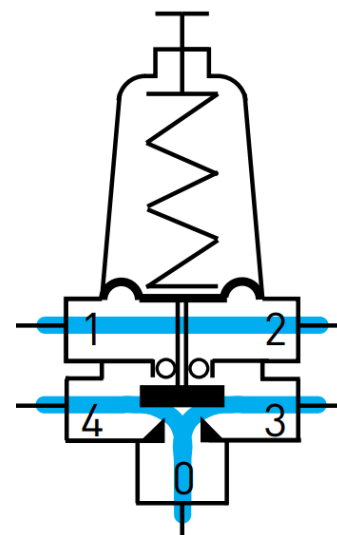
Modulating Open Regulated pressure higher than setting: 4 \leftrightarrow 3 \leftrightarrow 0
