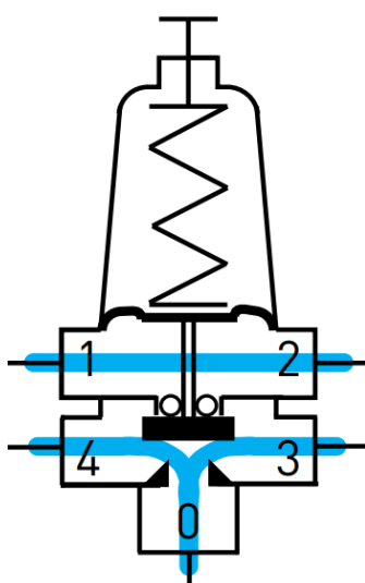
Stable Position Regulated pressure equal to setting: 4 \leftrightarrow 3 \leftrightarrow 0 controlled passage
