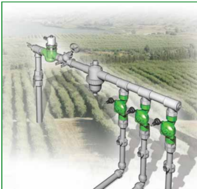
[1] BERMAD Model IR-430-50-KXZ opens upon pressure drop command, sustains supply system pressure, and controls laterals and distribution line fill-up.
