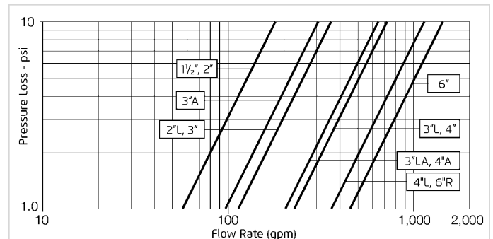
2-Way circuit "Added Head Loss" (for "V" below 6.5 f/s): 4.5 psi
