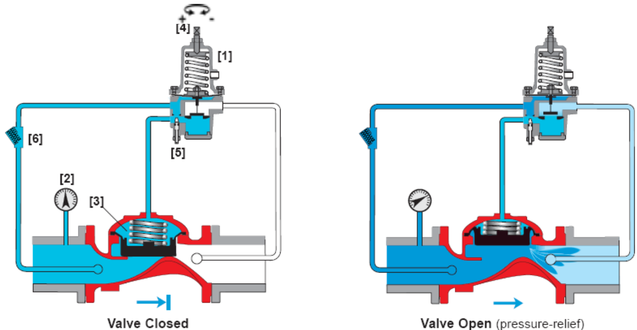
Figure 2: Operation Drawing
