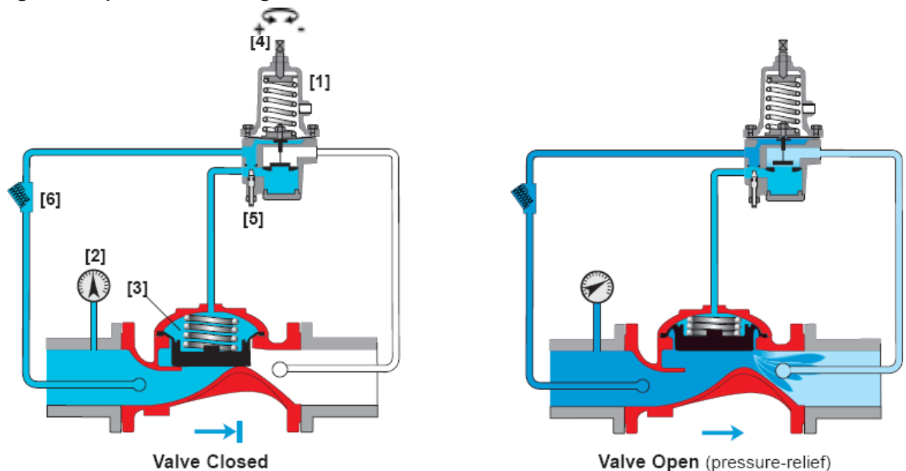
Figure 2: Operation Drawing
