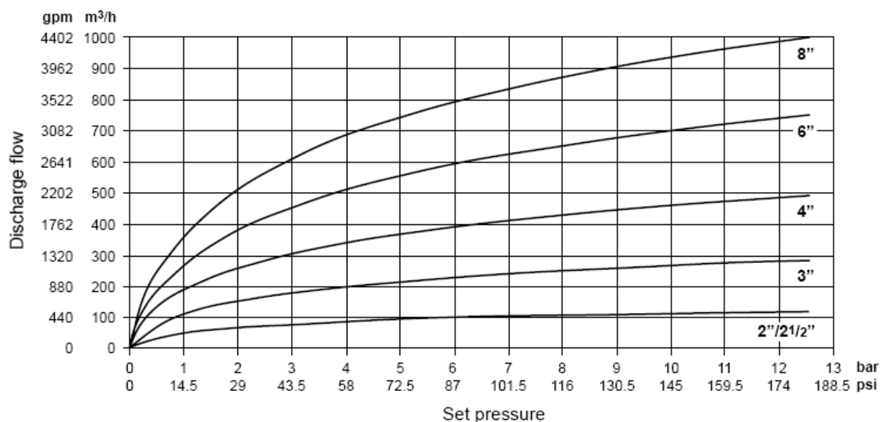
Figure 3: Discharge Chart
