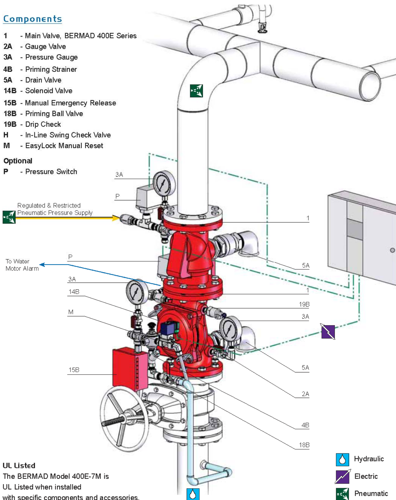
Figure 1: Installation Drawing
