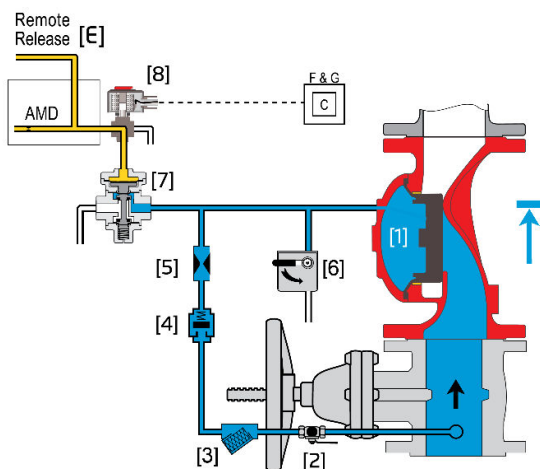
Figure 1 - Valve closed (NORMAL conditions)
