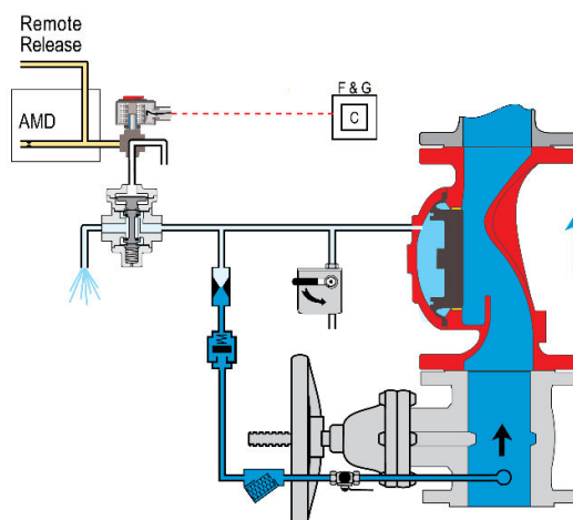
Figure 2 - Valve opened (FIRE conditions)
