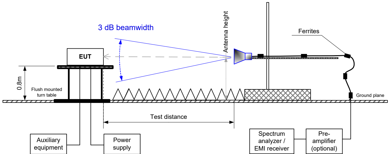
Figure 7.1.2 Setup for radiated emission measurements in semi anechoic chamber above 1 GHz, table-top EUT
