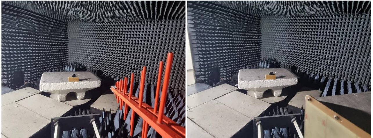
Photograph 8.2.2 Setup for radiated immunity to RF electromagnetic field test, EUT view
