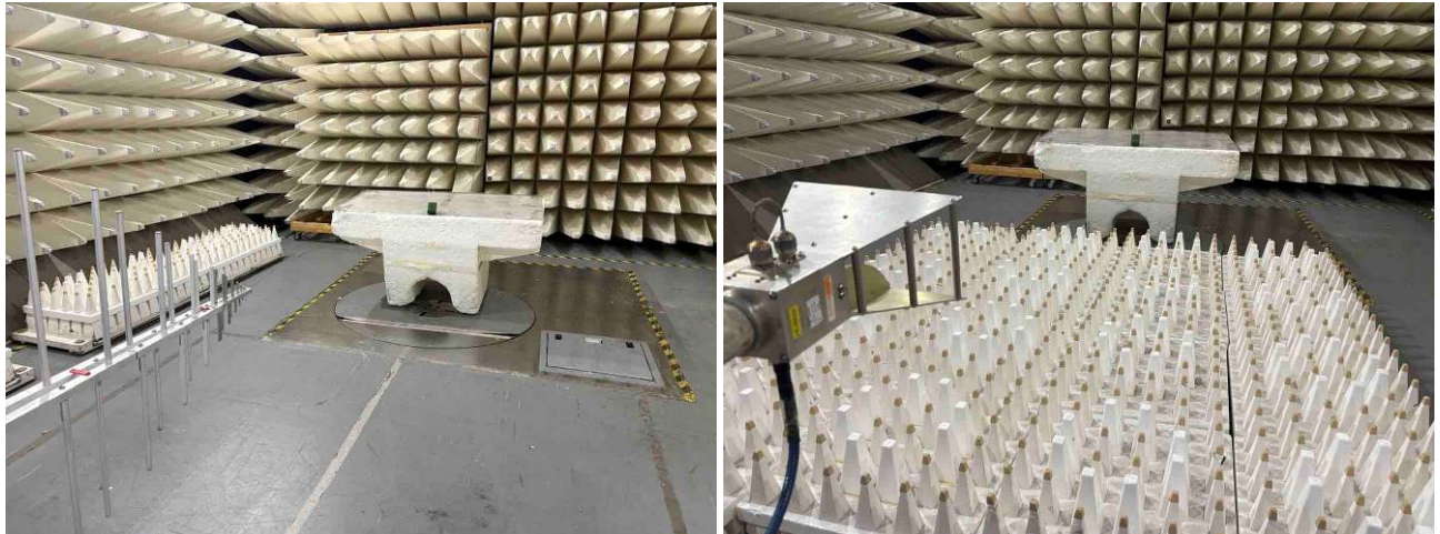
Photograph 7.1.2 Setup for radiated emission measurements, EUT view
