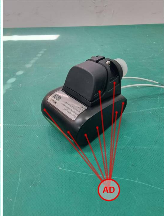
Photograph 8.1.2 Setup for immunity to ESD, EUT test points
