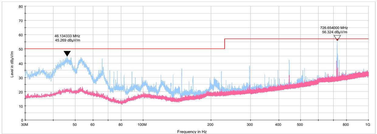
Plot 7.1.2 Radiated emission measurements in 1000 - 6000 MHz range, vertical & horizontal antenna polarization
