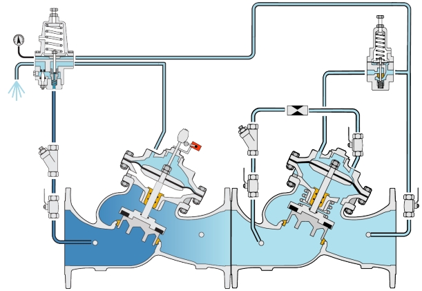
Watchdog Activated
