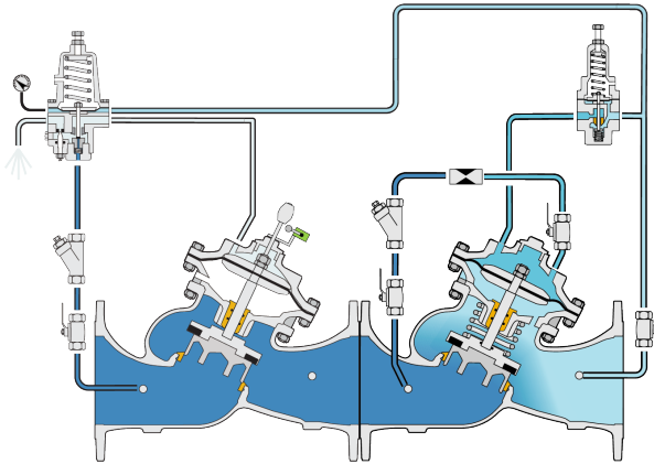
Watchdog Standing-By
