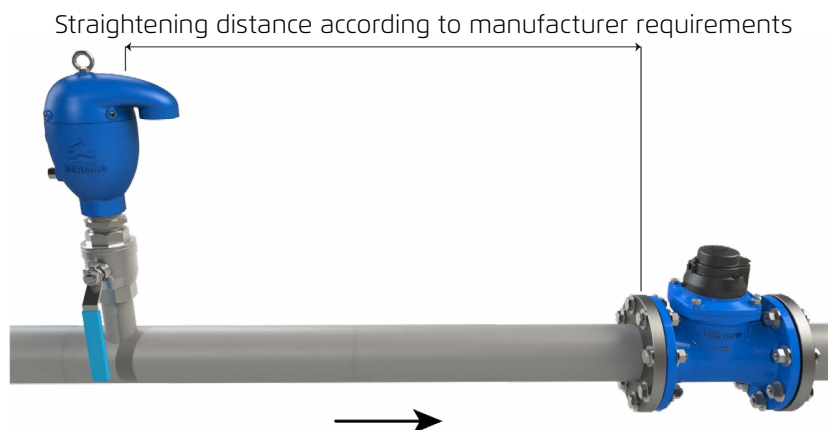
Picture 5.8 – Upstream of water meters
