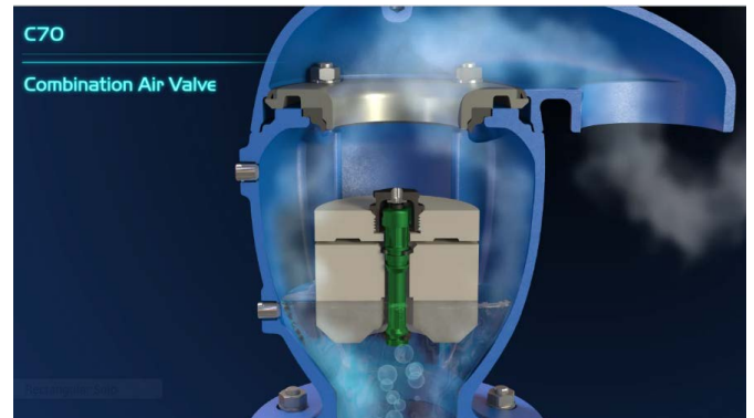
Picture 3.1 - C70, Air relief during pipeline filling
