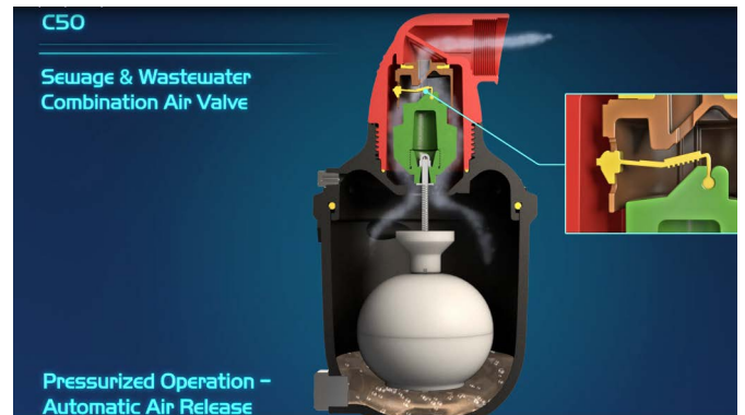
Picture 3.2 – C50, Automatic Air Release
